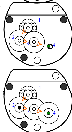
Figure 20: gears 1, 2 and 3 in place.
